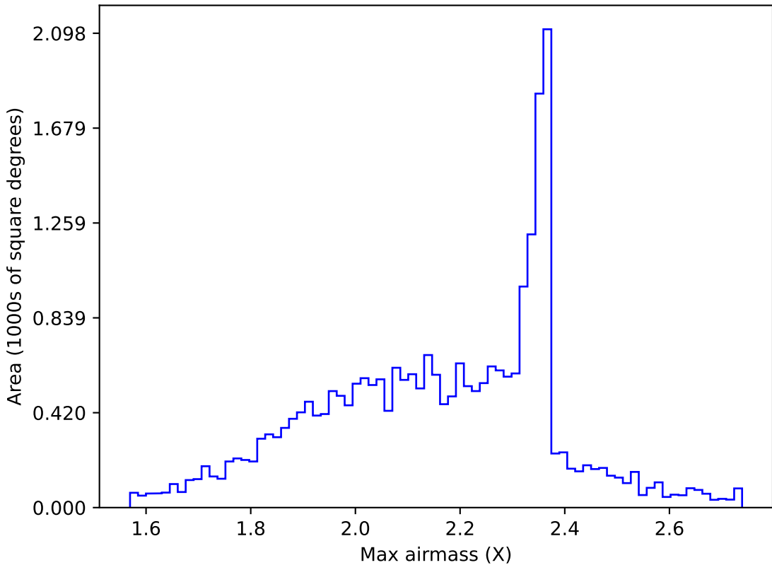
too_elab_r256_d3_ugrizy_v3.4_10yrs All sky g band: Max airmass
