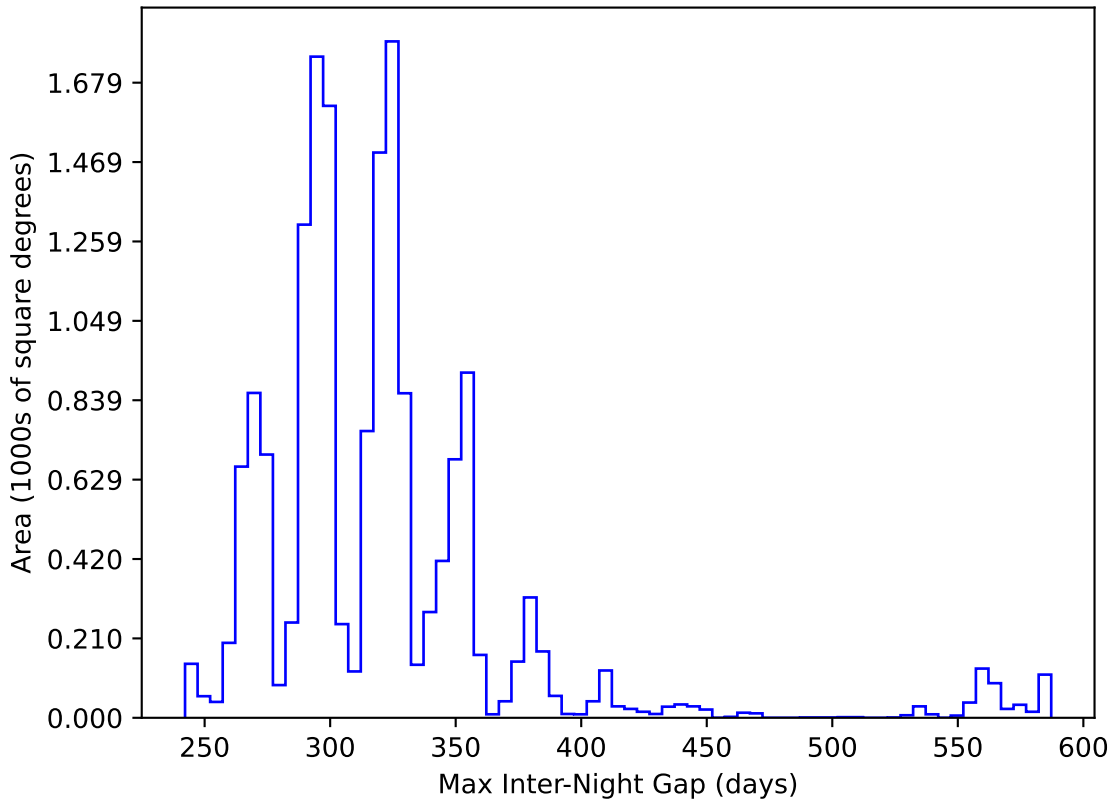
too_elab_r256_d3_ugrizy_v3.4_10yrs WFD y band: Max Inter-Night Gap
