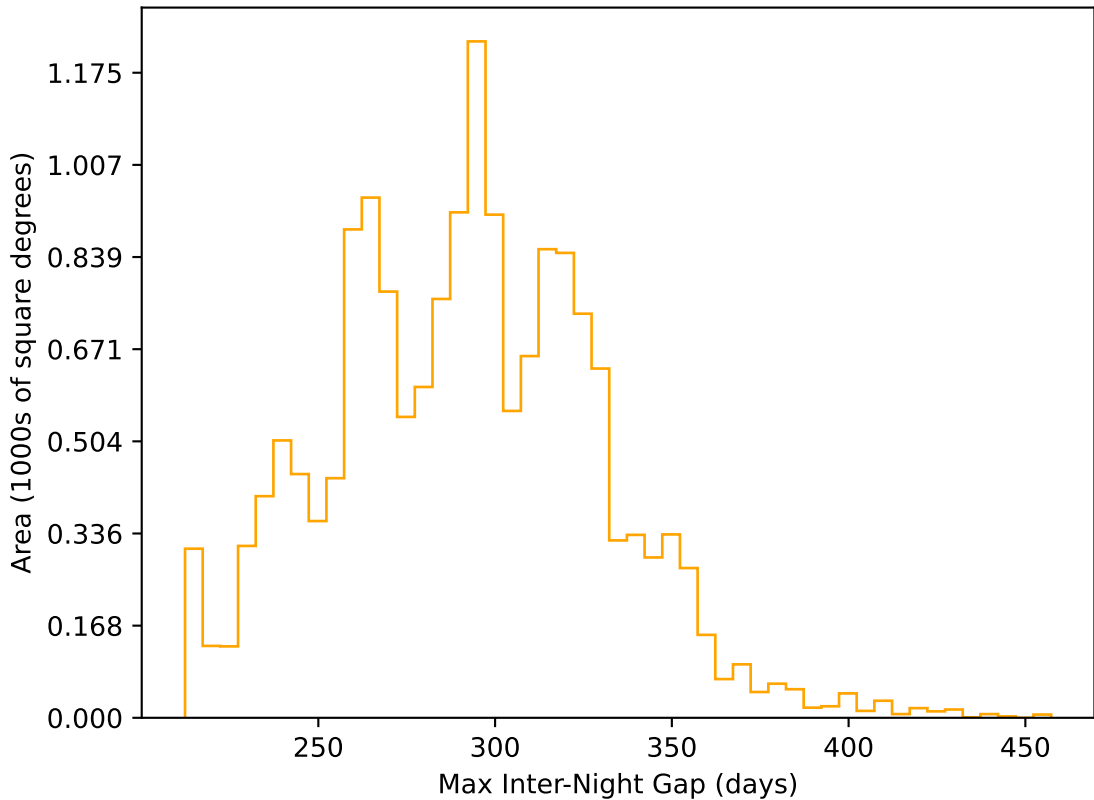
too_elab_r256_d3_ugrizy_v3.4_10yrs WFD r band: Max Inter-Night Gap
