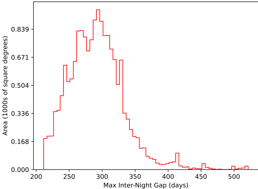
too_elab_r256_d3_ugrizy_v3.4_10yrs WFD i band: Max Inter-Night Gap
