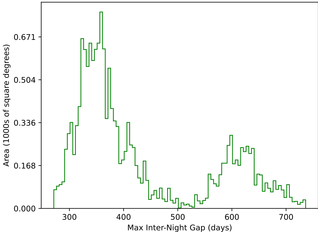
too_elab_r256_d3_ugrizy_v3.4_10yrs WFD g band: Max Inter-Night Gap
