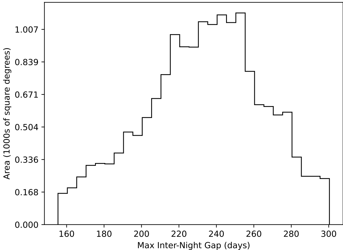
too_elab_r256_d3_ugrizy_v3.4_10yrs WFD all bands: Max Inter-Night Gap
