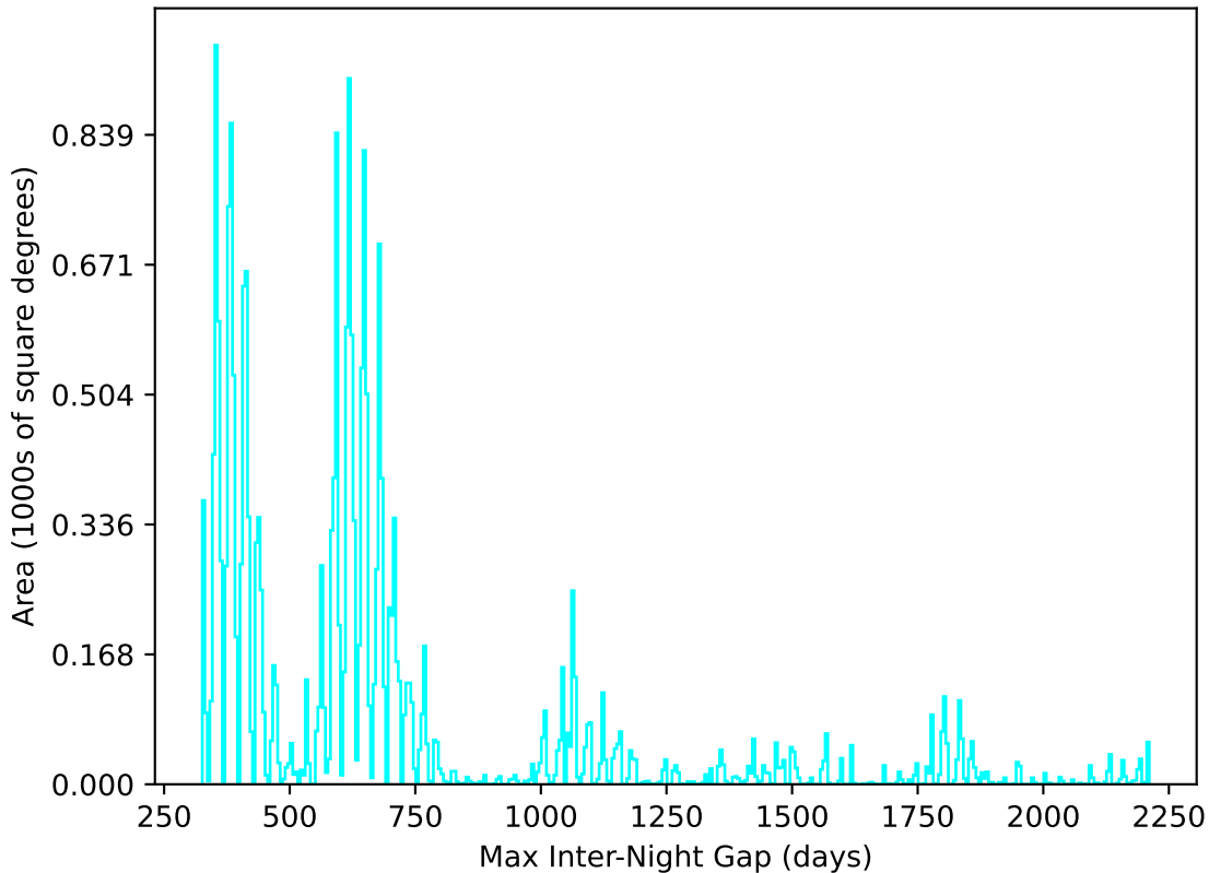
too_elab_r256_d3_ugrizy_v3.4_10yrs All sky u band: Max Inter-Night Gap
