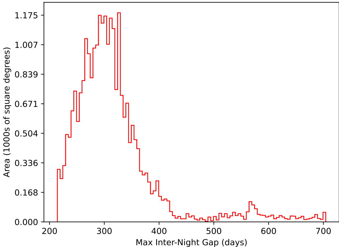
too_elab_r256_d3_ugrizy_v3.4_10yrs All sky i band: Max Inter-Night Gap
