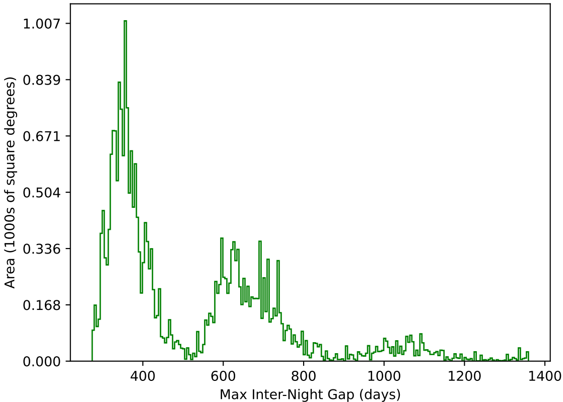
too_elab_r256_d3_ugrizy_v3.4_10yrs All sky g band: Max Inter-Night Gap
