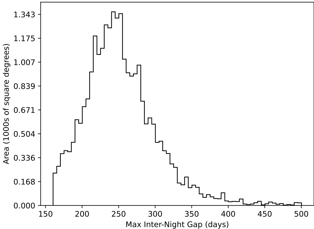
too_elab_r256_d3_ugrizy_v3.4_10yrs All sky all bands: Max Inter-Night Gap
