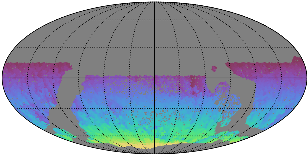
too_elab_r256_d3_ugrizy_v3.4_10yrs WFD all bands: Max HA
