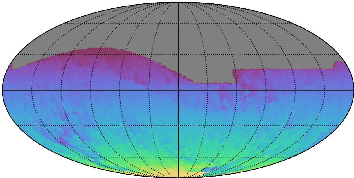
too_elab_r256_d3_ugrizy_v3.4_10yrs All sky all bands: Max HA
