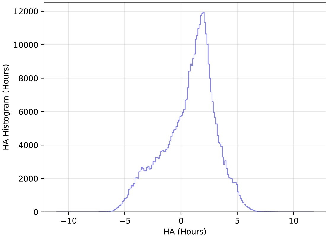
too_elab_r256_d3_ugrizy_v3.4_10yrs WFD z band: HA Histogram
