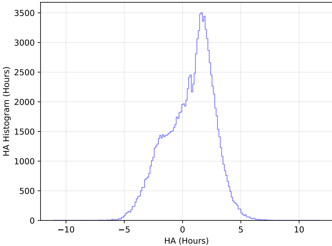
too_elab_r256_d3_ugrizy_v3.4_10yrs WFD u band: HA Histogram
