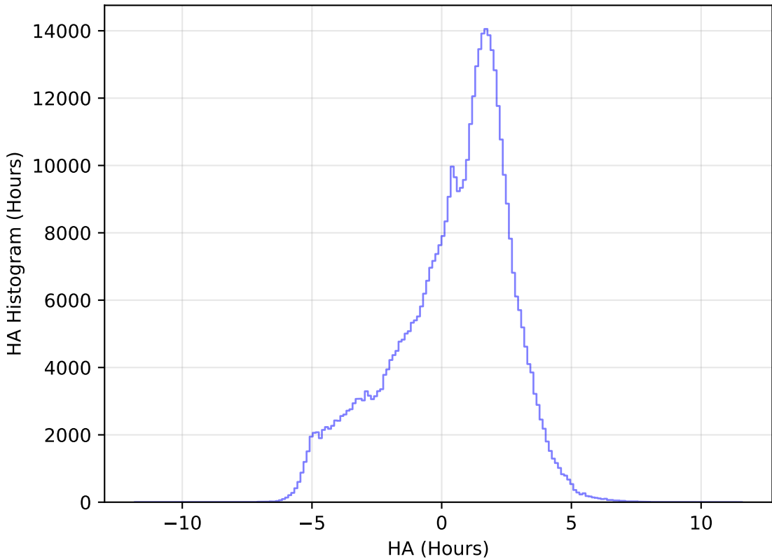
too_elab_r256_d3_ugrizy_v3.4_10yrs WFD r band: HA Histogram
