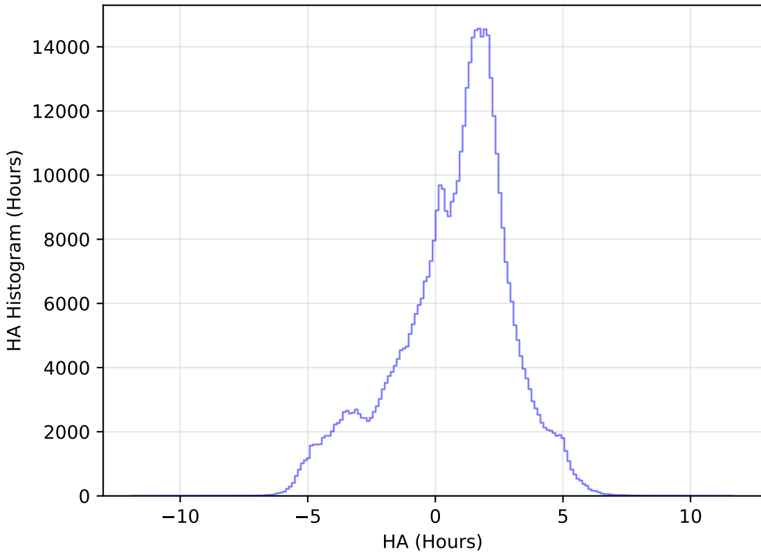
too_elab_r256_d3_ugrizy_v3.4_10yrs WFD i band: HA Histogram
