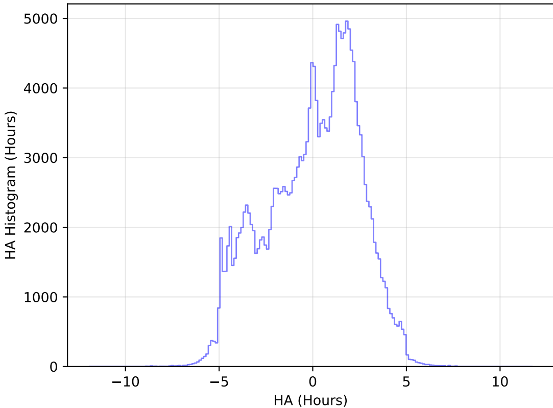
too_elab_r256_d3_ugrizy_v3.4_10yrs WFD g band: HA Histogram
