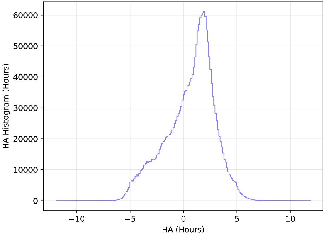
too_elab_r256_d3_ugrizy_v3.4_10yrs WFD all bands: HA Histogram
