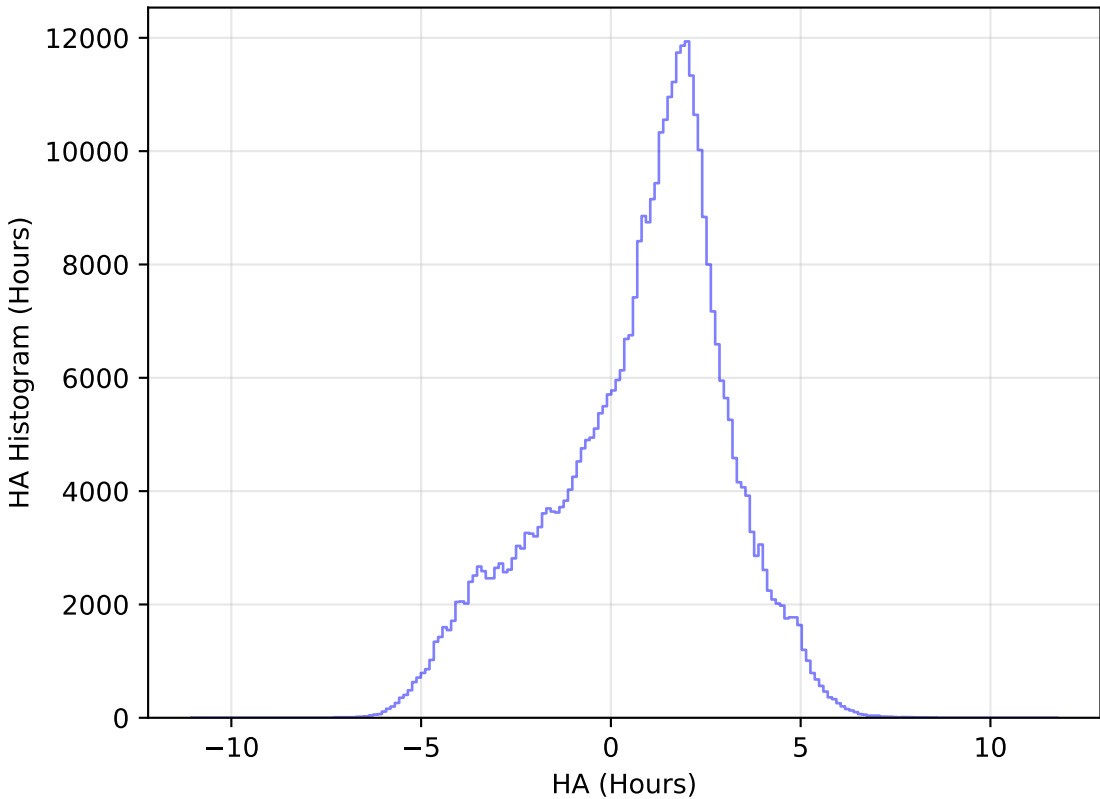
too_elab_r256_d3_ugrizy_v3.4_10yrs All sky z band: HA Histogram
