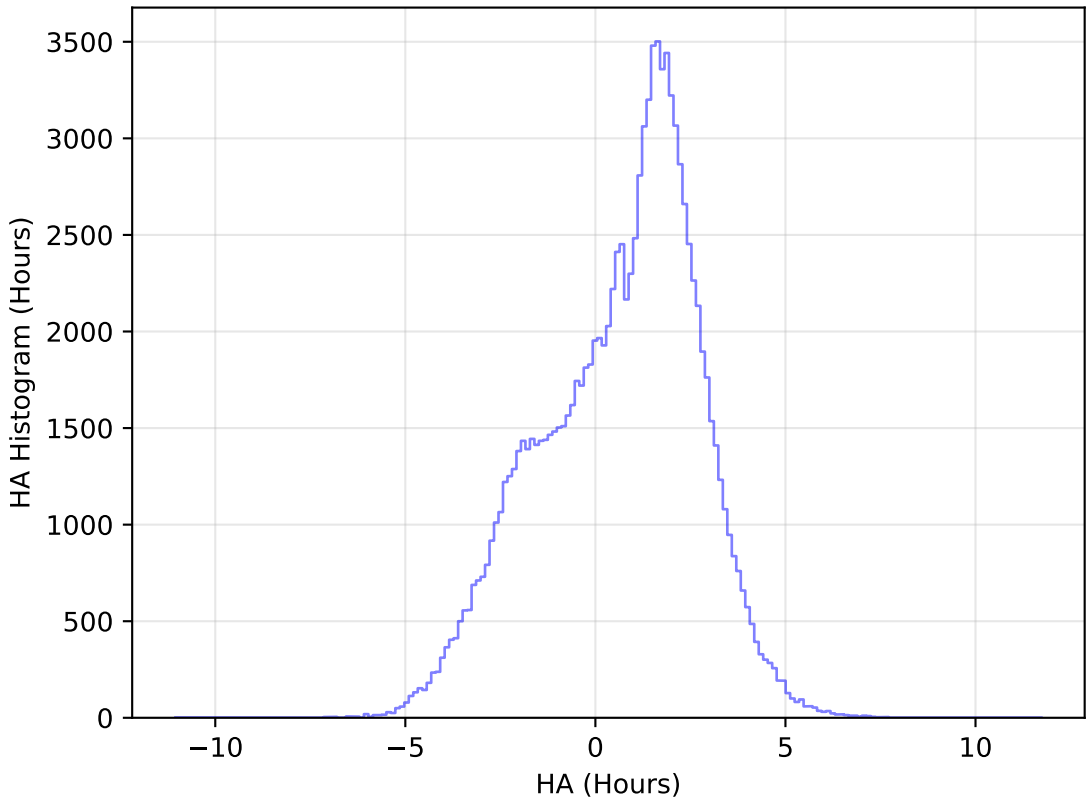
too_elab_r256_d3_ugrizy_v3.4_10yrs All sky u band: HA Histogram
