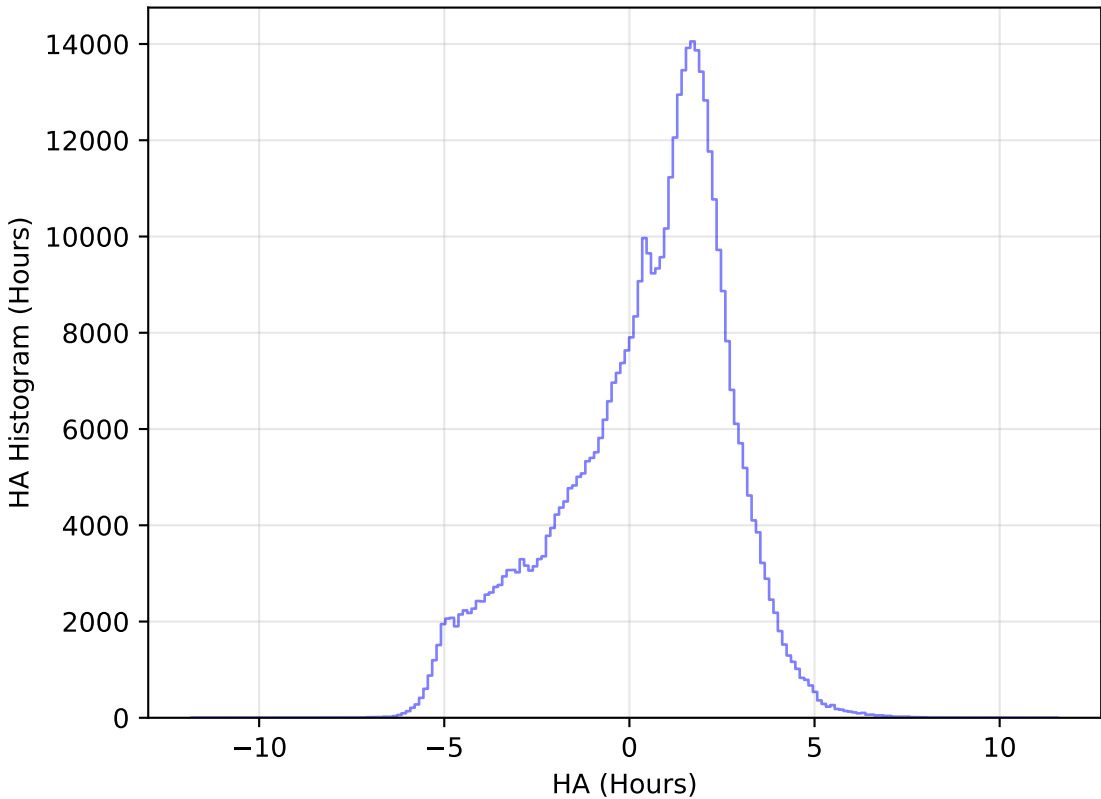
too_elab_r256_d3_ugrizy_v3.4_10yrs All sky r band: HA Histogram
