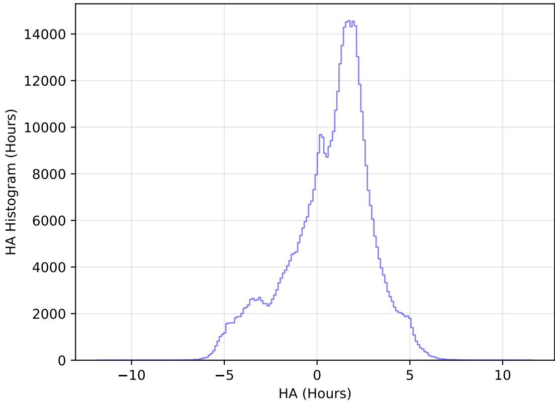
too_elab_r256_d3_ugrizy_v3.4_10yrs All sky i band: HA Histogram
