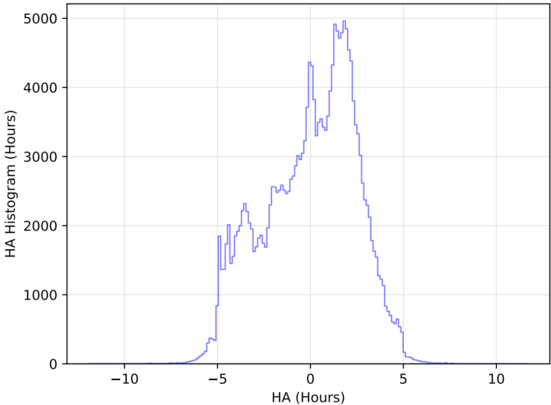
too_elab_r256_d3_ugrizy_v3.4_10yrs All sky g band: HA Histogram
