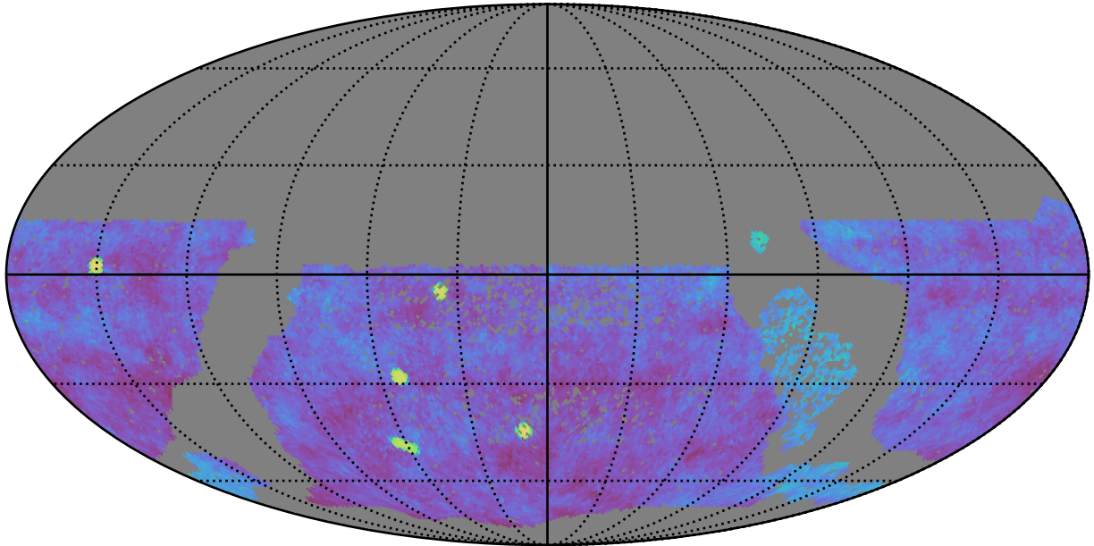
too_elab_r256_d3_ugrizy_v3.4_10yrs gri WFD: Fraction of visits in pairs (10-60 min)
