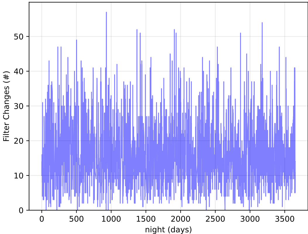
too_elab_r256_d3_ugrizy_v3.4_10yrs Per Night: Filter Changes
