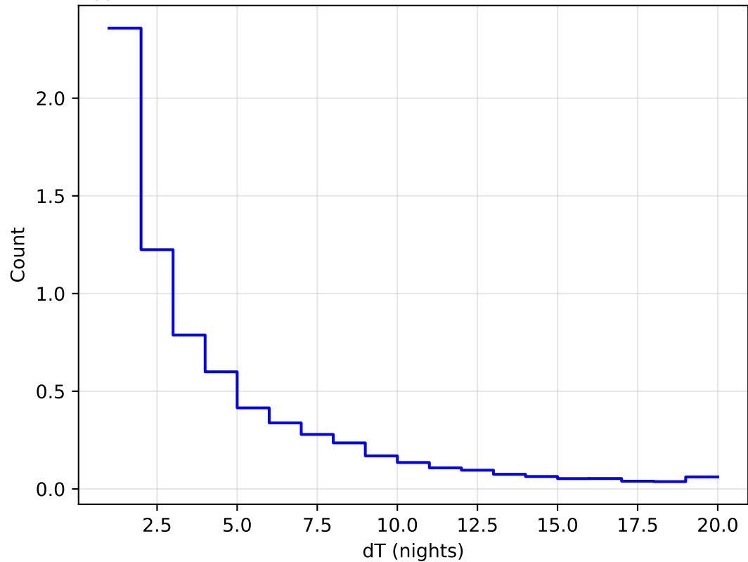
too_elab_r256_d3_ugrizy_v3.4_10yrs WFD all bands: DeltaNight Histogram
