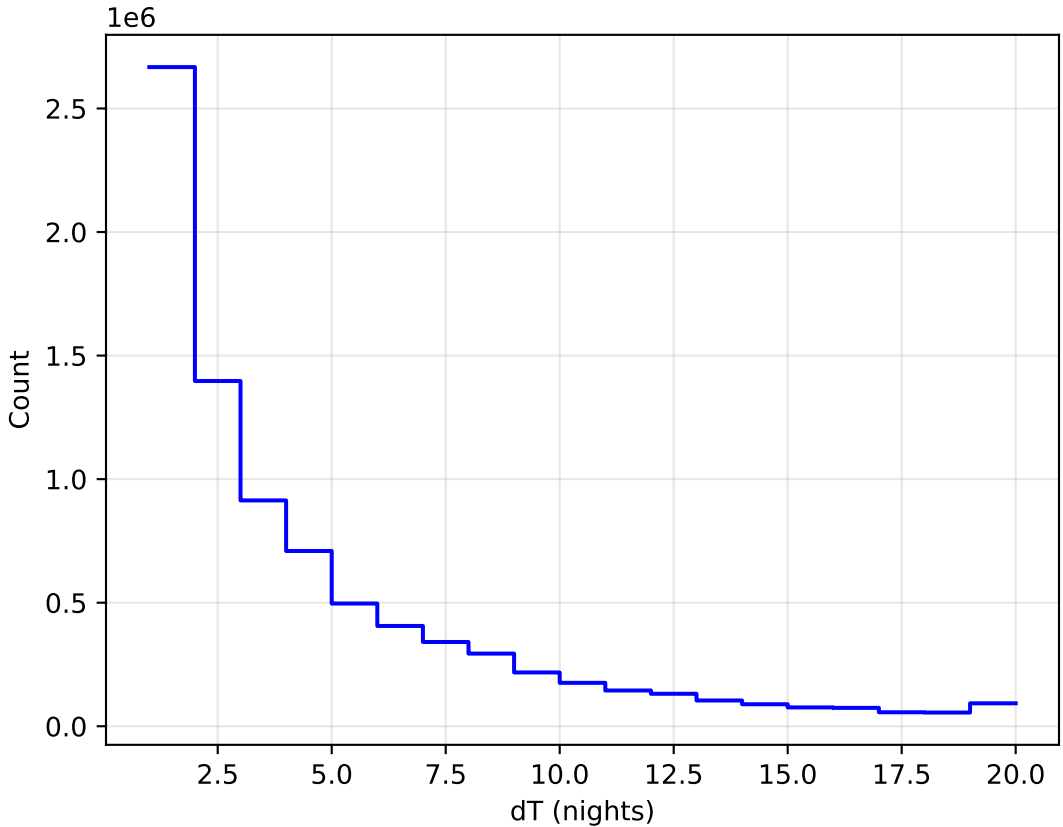
too_elab_r256_d3_ugrizy_v3.4_10yrs All sky all bands: DeltaNight Histogram
