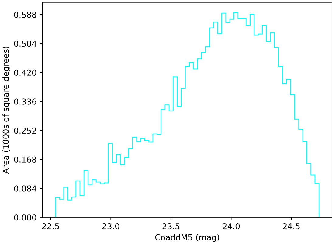
too_elab_r256_d3_ugrizy_v3.4_10yrs Yr 3-4 u band: CoaddM5
