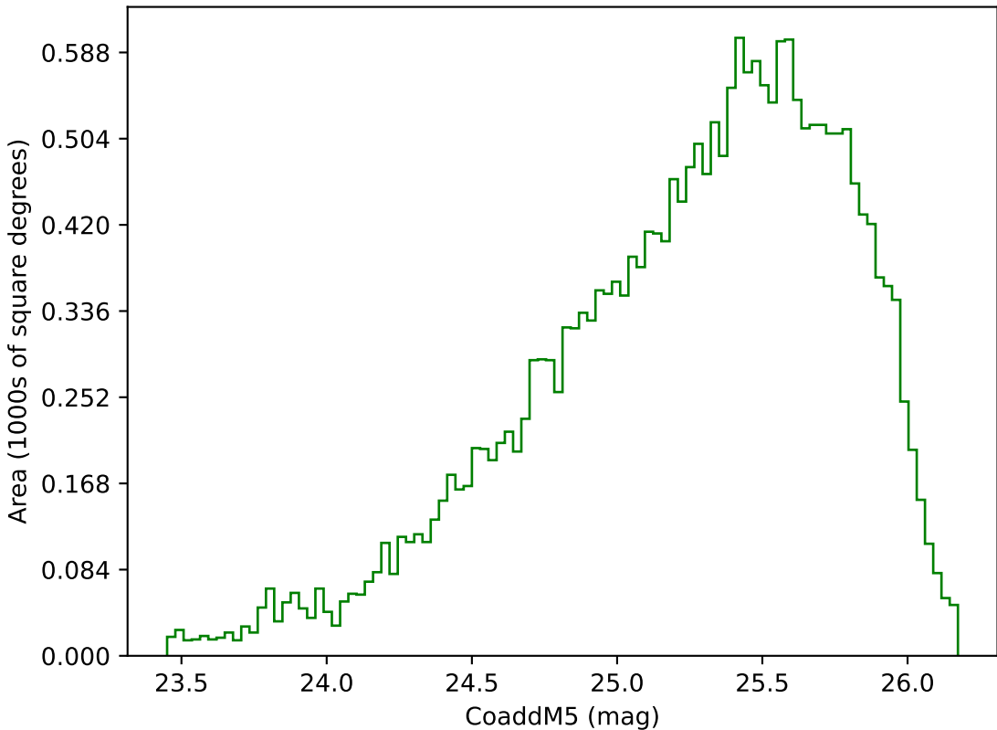
too_elab_r256_d3_ugrizy_v3.4_10yrs Yr 3-4 g band: CoaddM5
