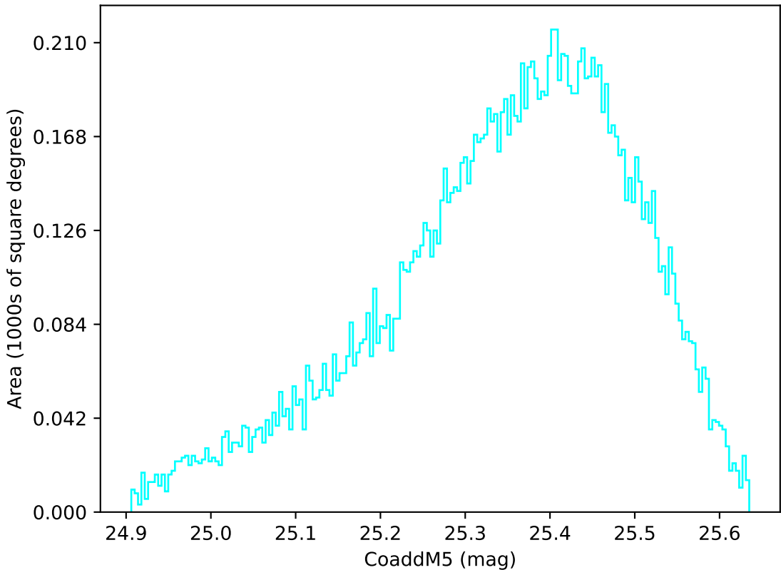
too_elab_r256_d3_ugrizy_v3.4_10yrs WFD u band: CoaddM5
