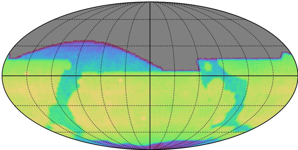
too_elab_r256_d3_ugrizy_v3.4_10yrs All sky i band: CoaddM5
