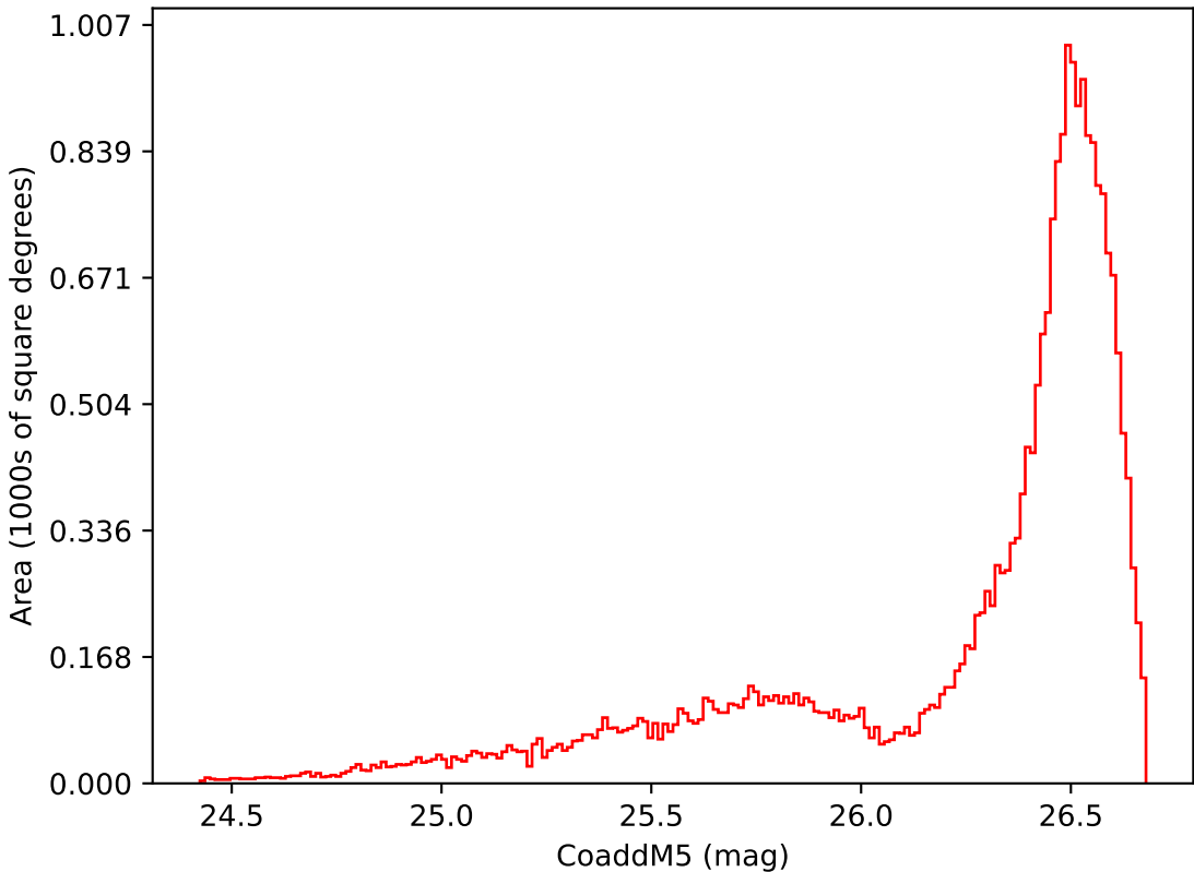
too_elab_r256_d3_ugrizy_v3.4_10yrs All sky i band: CoaddM5
