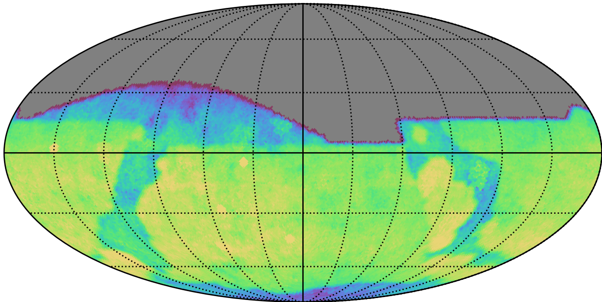
too_elab_r256_d3_ugrizy_v3.4_10yrs All sky g band: CoaddM5
