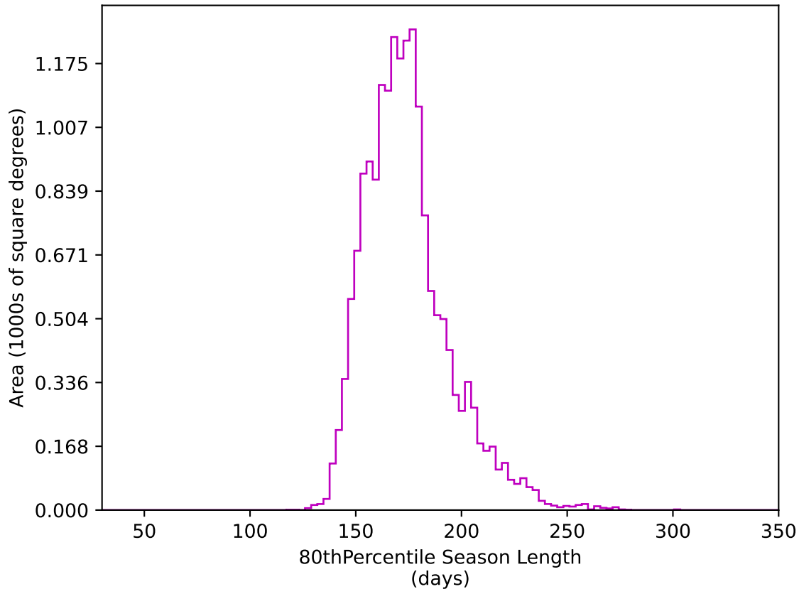
too_elab_r256_d3_ugrizy_v3.4_10yrs WFD z band: 80thPercentile Season Length
