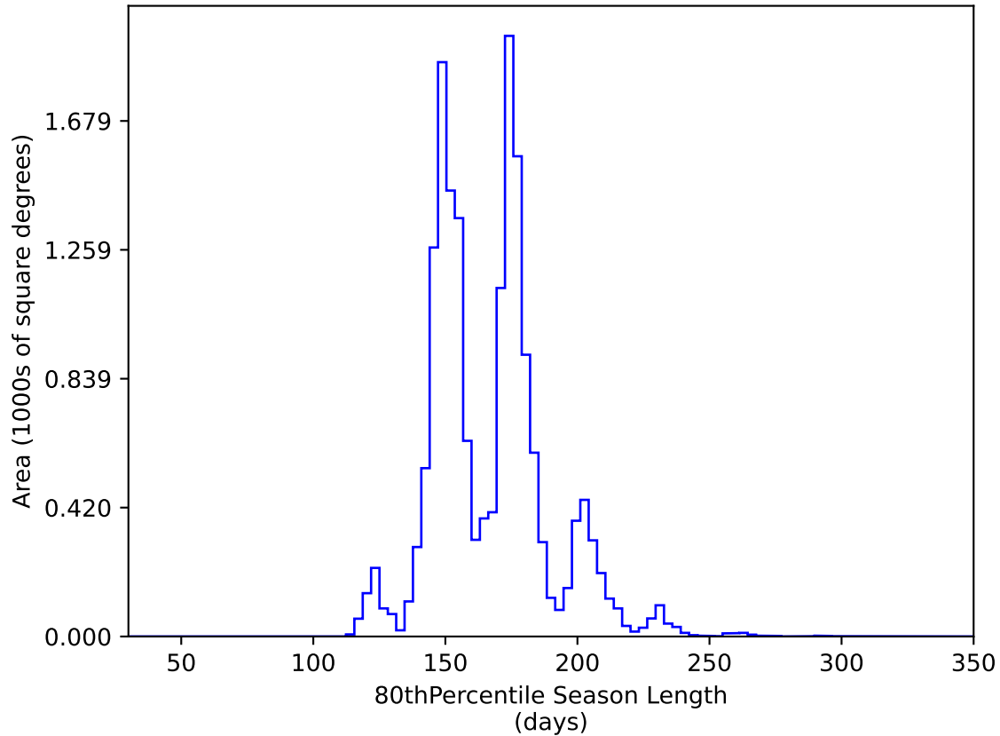
too_elab_r256_d3_ugrizy_v3.4_10yrs WFD y band: 80thPercentile Season Length
