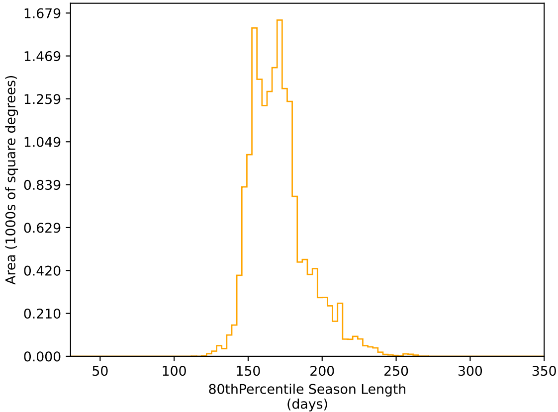
too_elab_r256_d3_ugrizy_v3.4_10yrs WFD r band: 80thPercentile Season Length
