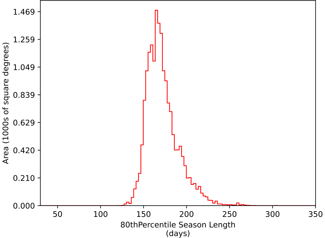
too_elab_r256_d3_ugrizy_v3.4_10yrs WFD i band: 80thPercentile Season Length
