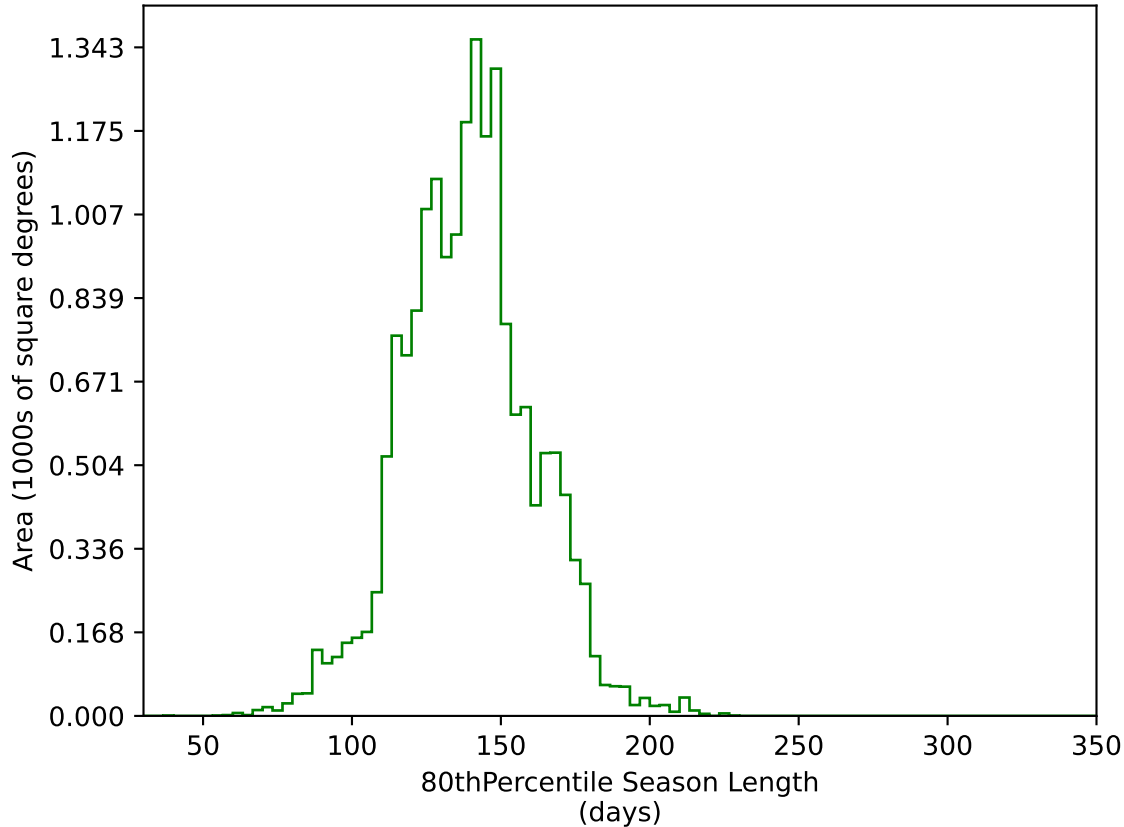
too_elab_r256_d3_ugrizy_v3.4_10yrs WFD g band: 80thPercentile Season Length
