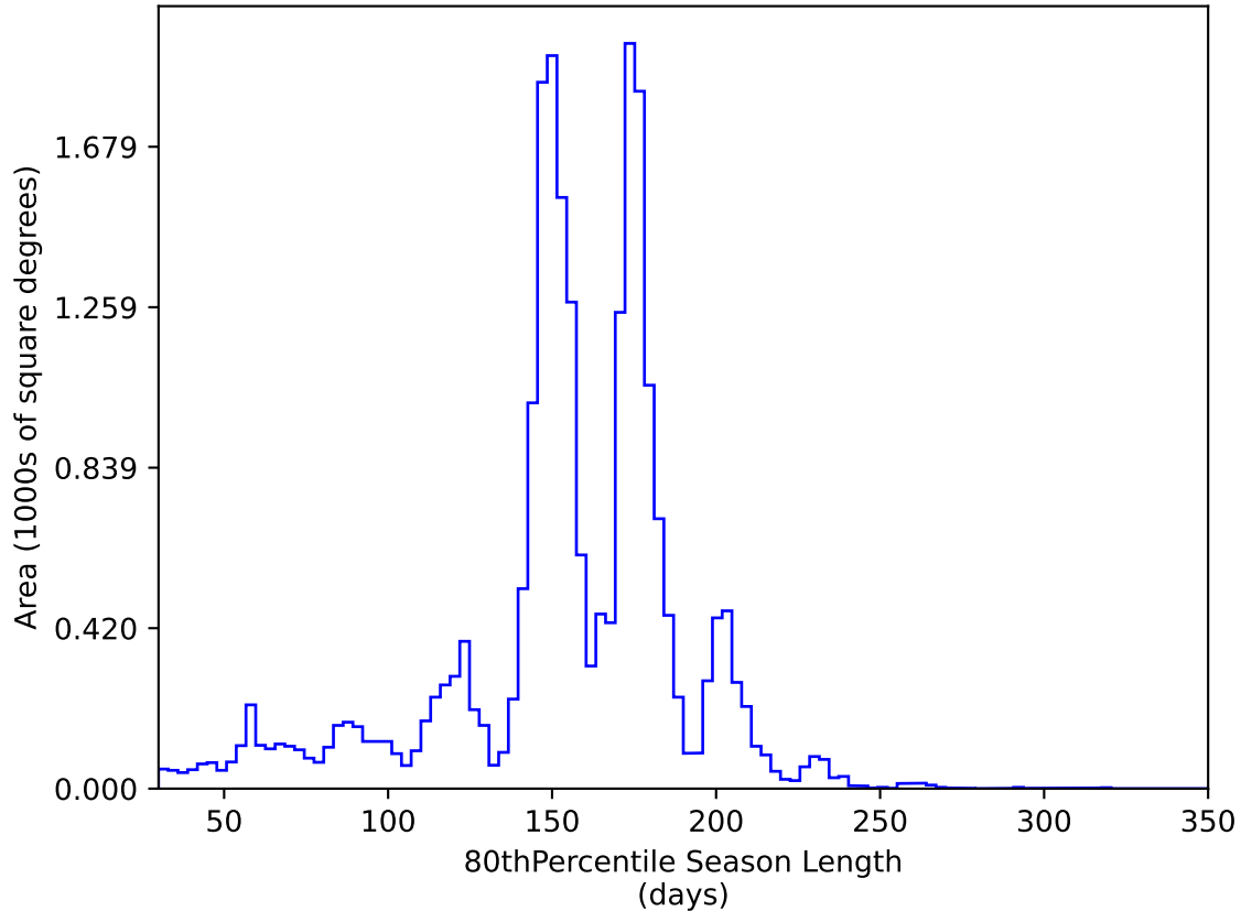
too_elab_r256_d3_ugrizy_v3.4_10yrs All sky y band: 80thPercentile Season Length
