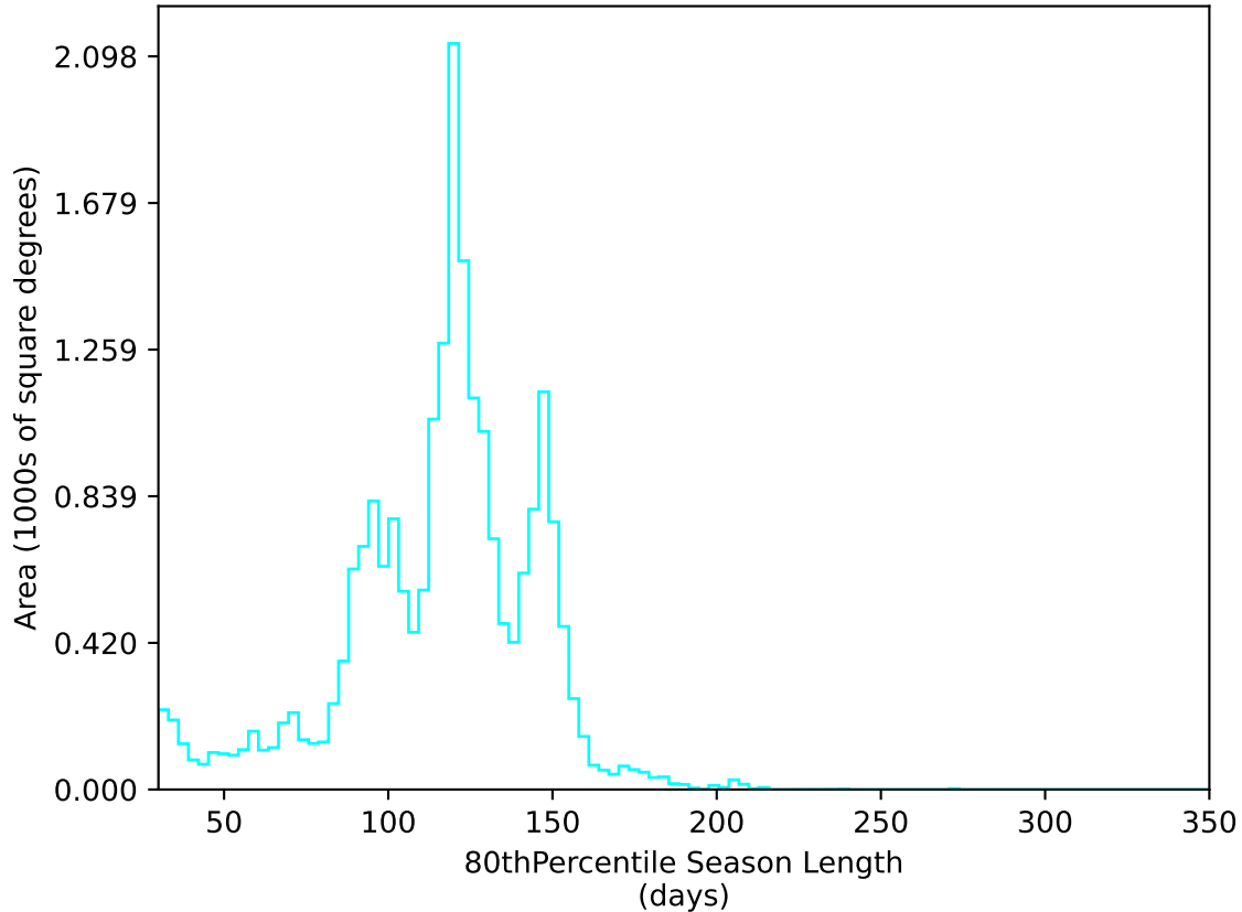
too_elab_r256_d3_ugrizy_v3.4_10yrs All sky u band: 80thPercentile Season Length
