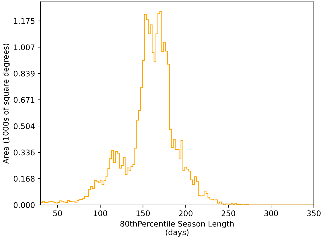
too_elab_r256_d3_ugrizy_v3.4_10yrs All sky r band: 80thPercentile Season Length
