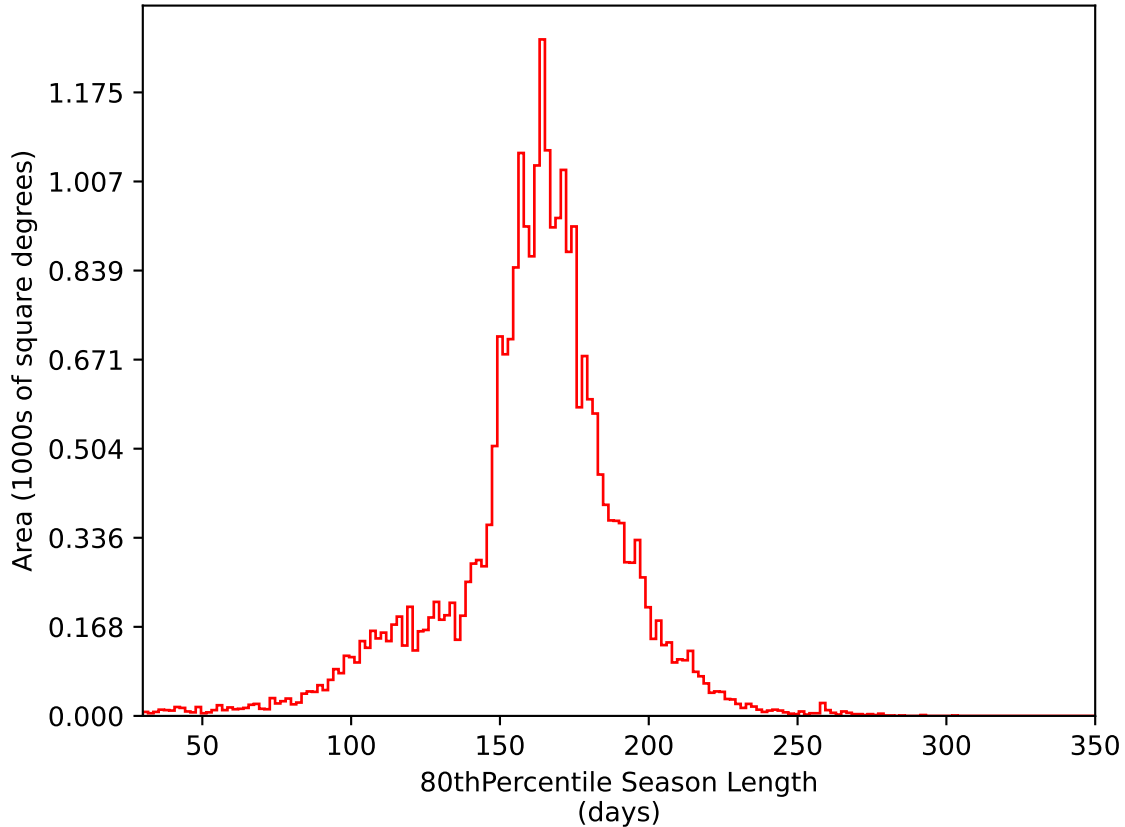
too_elab_r256_d3_ugrizy_v3.4_10yrs All sky i band: 80thPercentile Season Length
