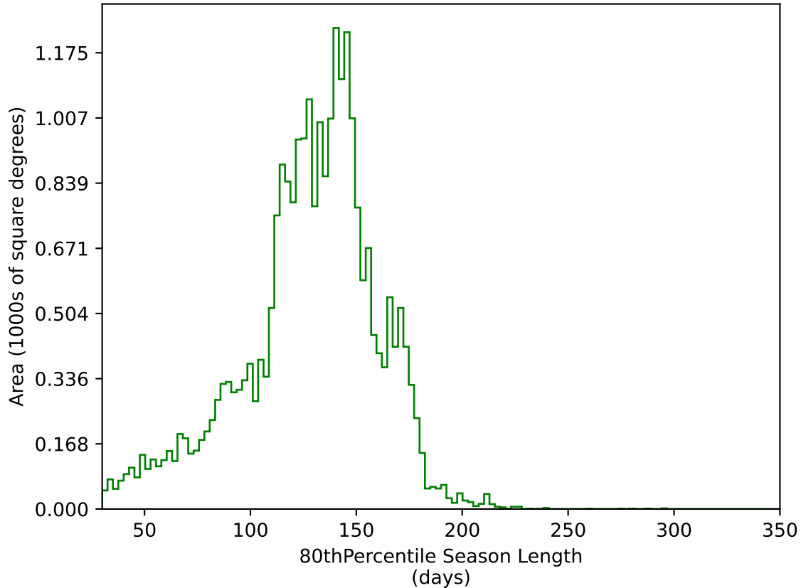
too_elab_r256_d3_ugrizy_v3.4_10yrs All sky g band: 80thPercentile Season Length
