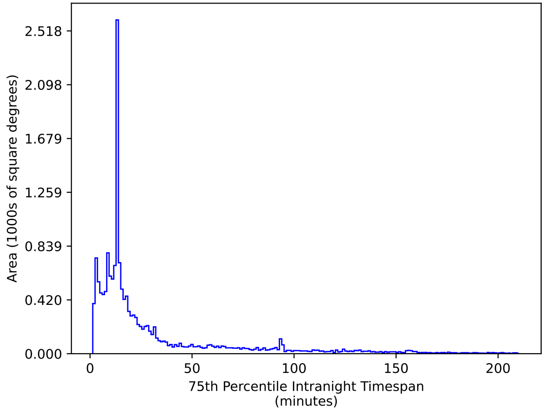
too_elab_r256_d3_ugrizy_v3.4_10yrs WFD z band: 75th Percentile Intranight Timespan
