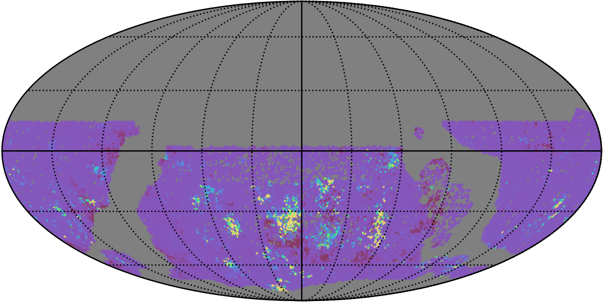
too_elab_r256_d3_ugrizy_v3.4_10yrs WFD ug bands: 75th Percentile Intranight Timespan
