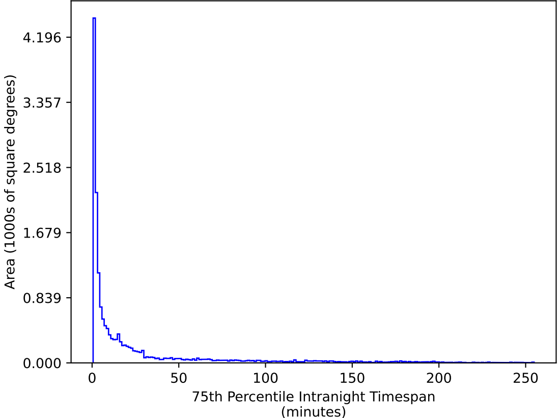
too_elab_r256_d3_ugrizy_v3.4_10yrs WFD u band: 75th Percentile Intranight Timespan
