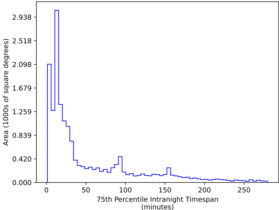
too_elab_r256_d3_ugrizy_v3.4_10yrs WFD r band: 75th Percentile Intranight Timespan
