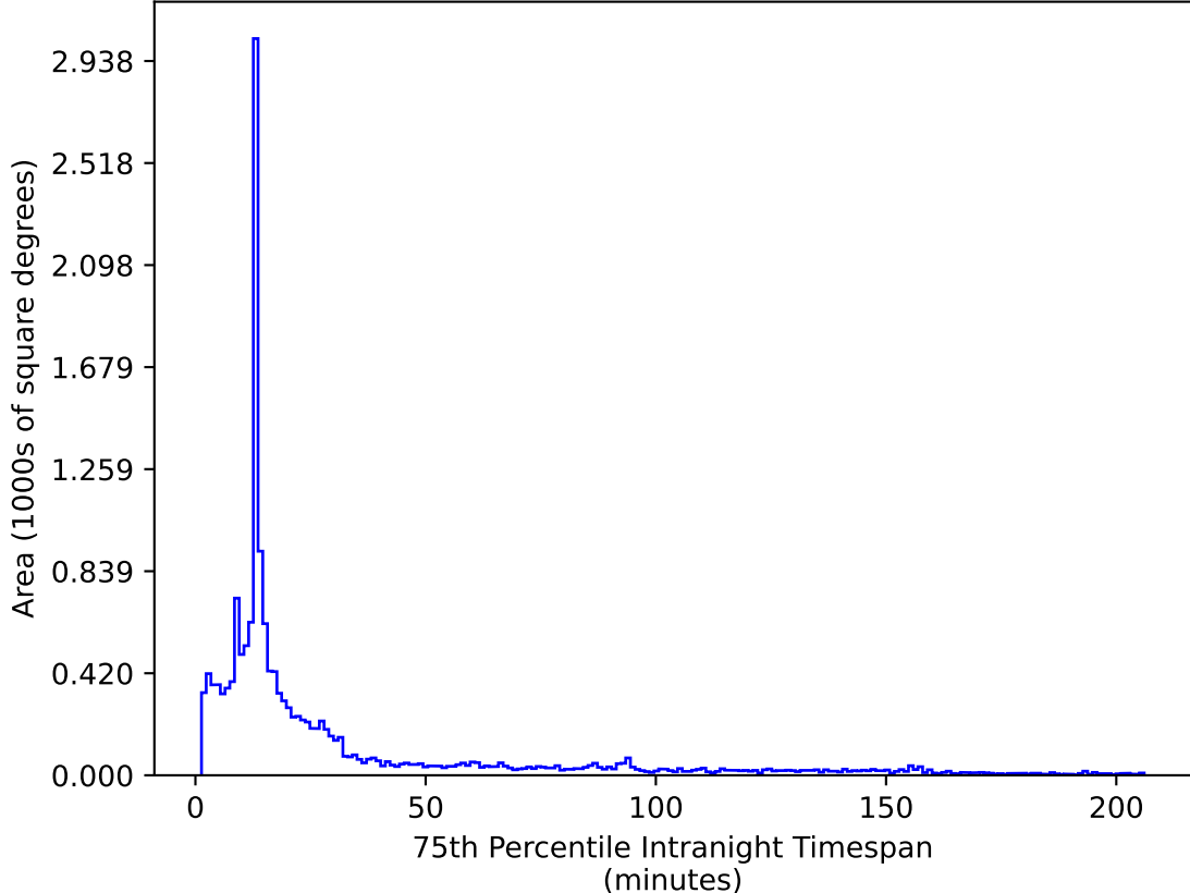
too_elab_r256_d3_ugrizy_v3.4_10yrs WFD i band: 75th Percentile Intranight Timespan
