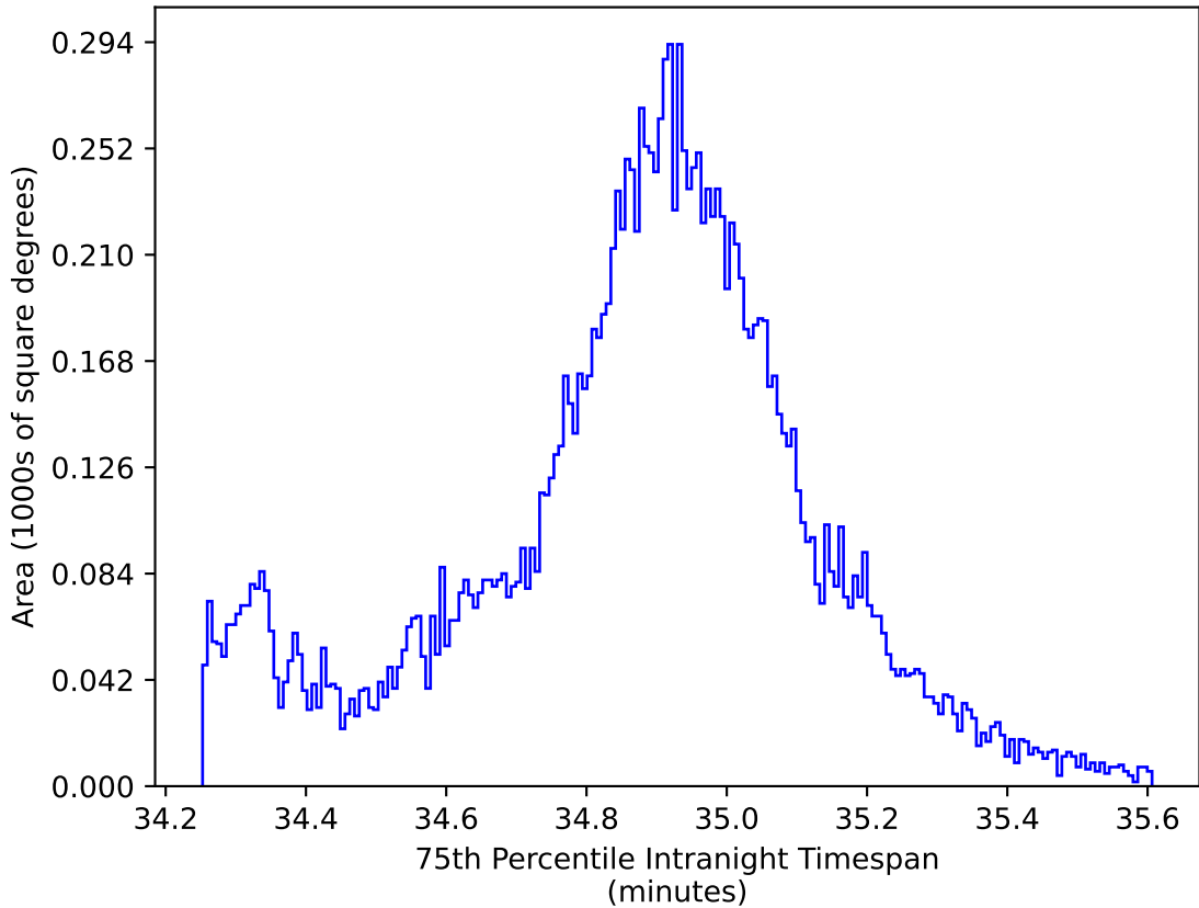
too_elab_r256_d3_ugrizy_v3.4_10yrs WFD all bands: 75th Percentile Intranight Timespan
