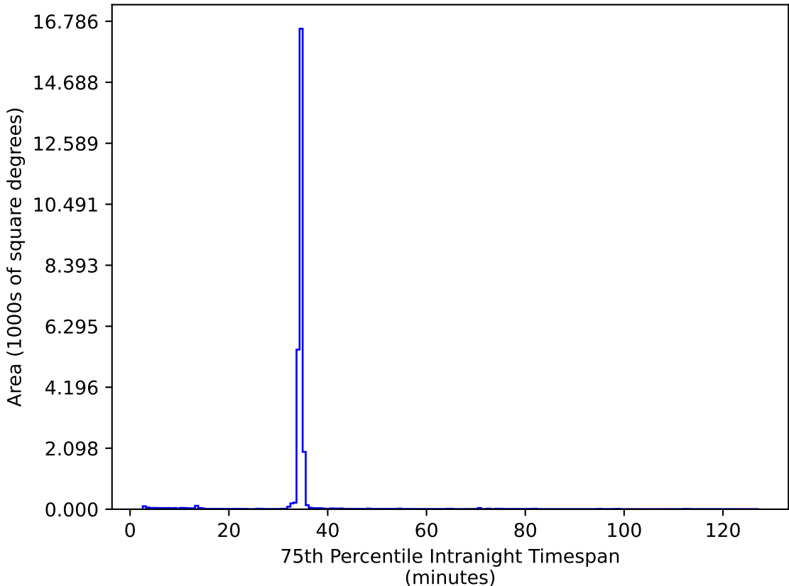
too_elab_r256_d3_ugrizy_v3.4_10yrs All sky zy bands: 75th Percentile Intranight Timespan
